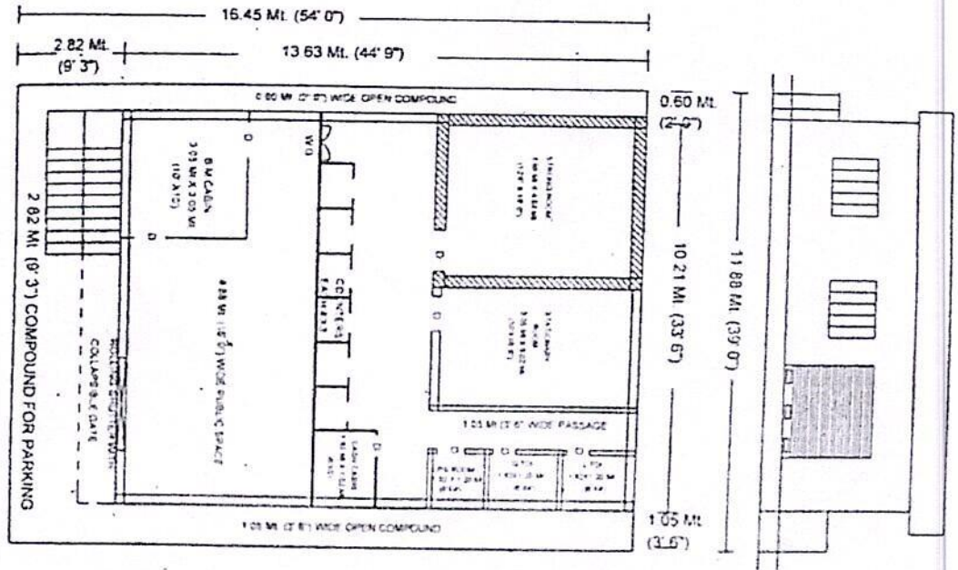
PROPOSED PLAN OF GROUND FLOOR
