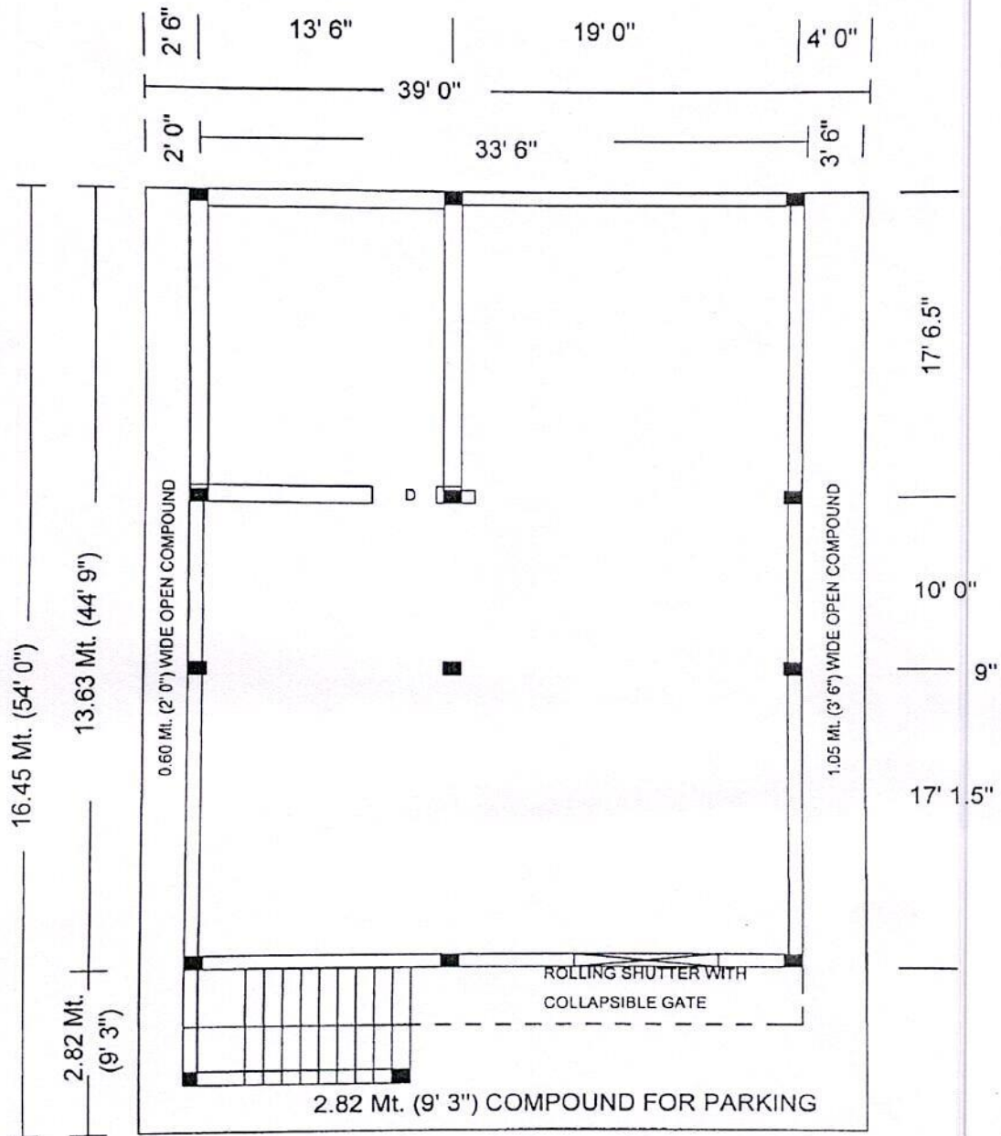
PROPOSED PLAN OF GROUND FLOOR
